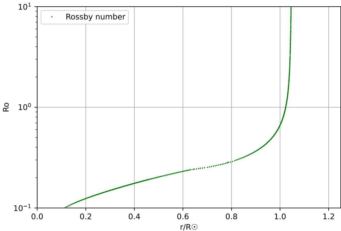
Rossby number, profile 111, age 2.33 \times 10^7
